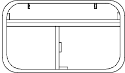
Standard Hopper/Slider window with concealed fixings and 4mm toughened glass to BS6206A Top glass hopper and bottom half fixed and half slider. 3" radius corners all round.
