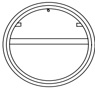
Wesley Aluminium Clamp on Porthole with Drop Back Vent. 4mm toughened glass to BS6206A.
