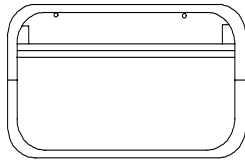
Wesley Clamp on Standard Top Hopper window with radius corners all round. 4mm toughened glass to BS6206A. All corners 85mm radius.
