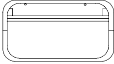
Standard Hopper window with concealed fixings and 4mm toughened glass to Bs6206A. 3" radius corners all round
