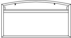
Hopper Arched Top window with concealed fixings and 4mm toughened glass to BS6206A Mitred top corners and bottom corners Available with radius bottom corners.
