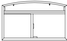
Hopper 'Slider Arched Top window with concealed fixings and 4mm toughened glass to BS6206A. Top hopper glass and bottom slider. Mitred top corners and 3" radius bottom corners.
