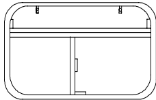
Wesley Clamp on Hopper/Slider window with radius corners all round. Top Hopper window with one fixed and one sliding bottom pane. 4mm toughened glass to BS6206A. All corners 85mm radius.
